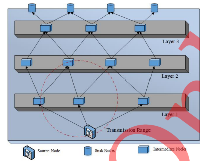
Fig. 1. Schematic Diagram of Multi-Layered UWMSN
